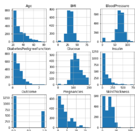
Fig 4: label outcome
